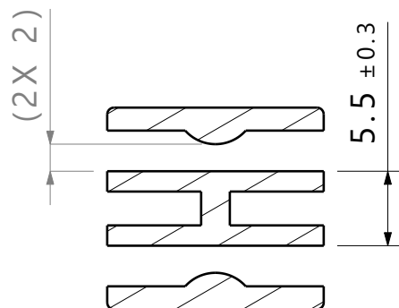
COUPLER ALONE
