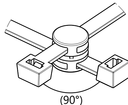
MAX ANGLE SEE NOTE 3
